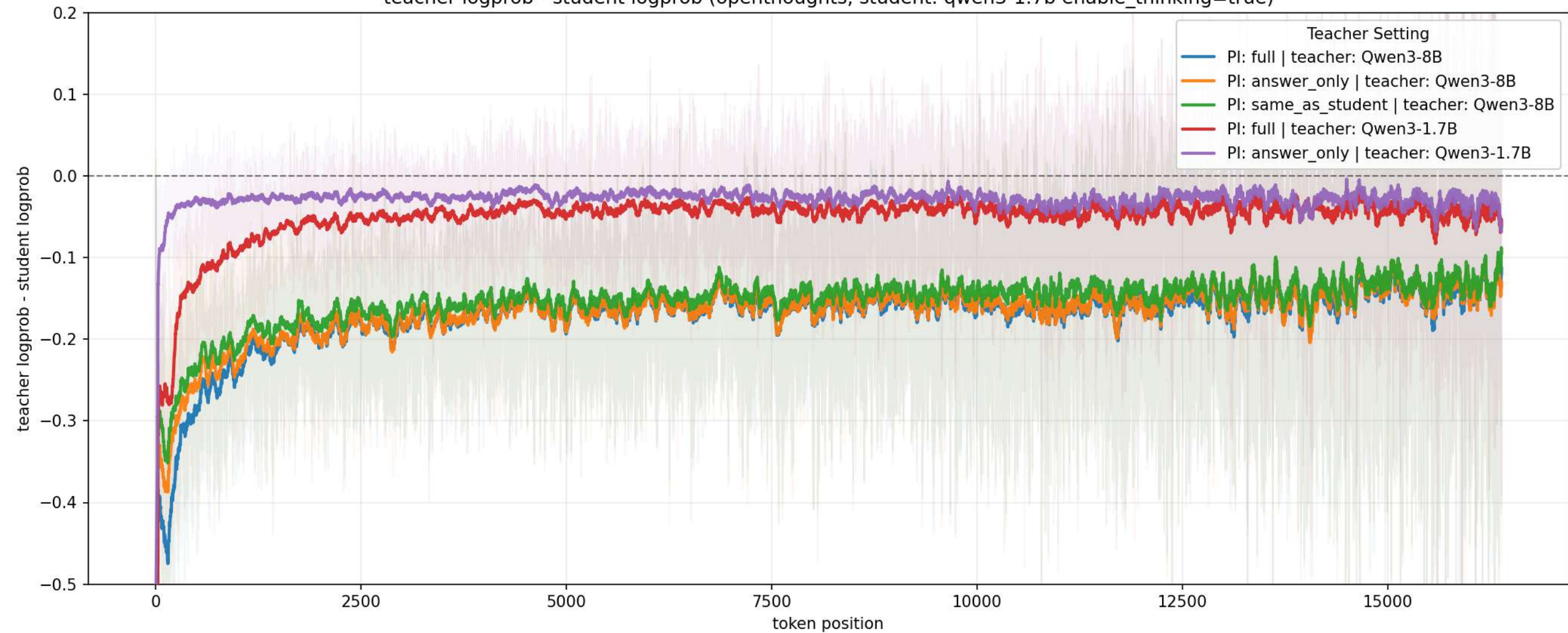
teacher logprob - student logprob (openthoughts, student: qwen3-1.7b enable_thinking=true)
